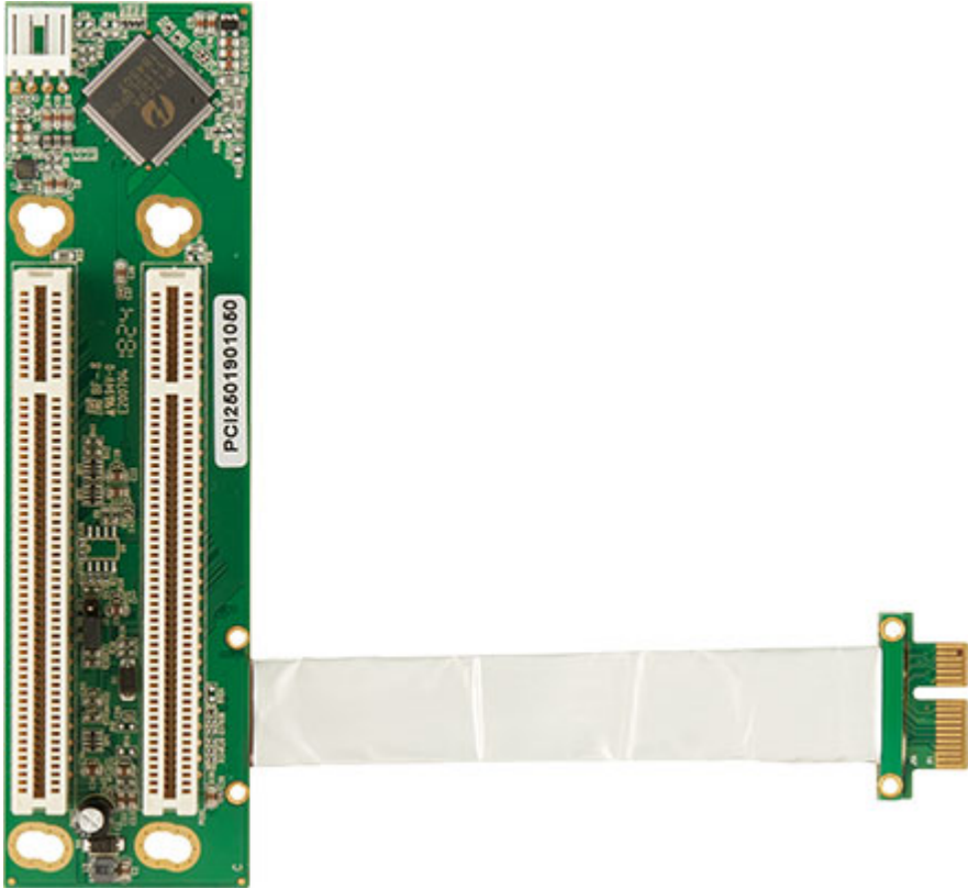
PCIex1 to 2PCI riser card, L=100 mm
